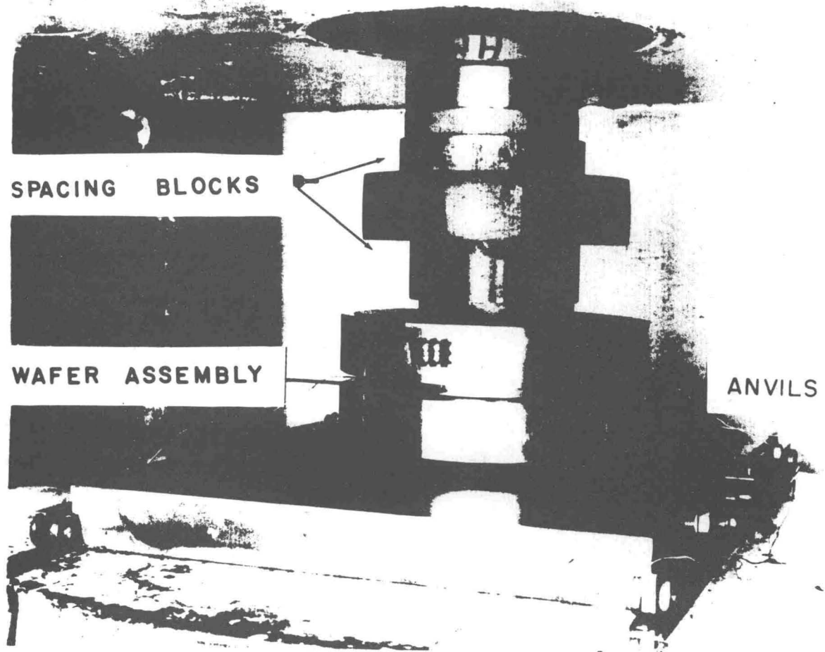
FIG. 5 COMPLETE ASSEMBLY OF CONFINED WAFER COMPRESSION SYSTEM
